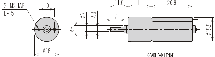
GEARHEAD LENGTH
