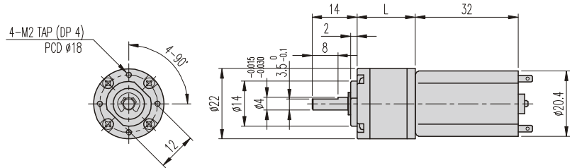
GEARHEAD LENGTH
