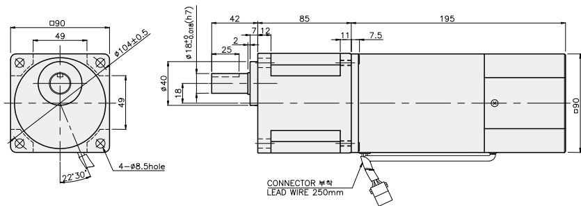
K9IP180F□-SU + K9P□BU
