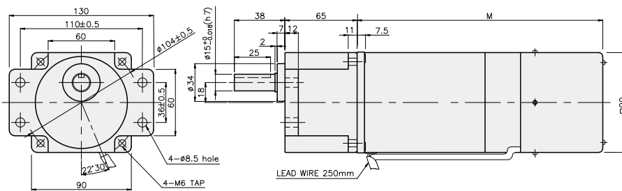
K9RP120F□-D + K9P□BF
