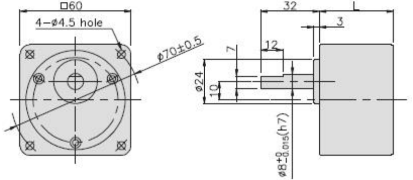
DG60-F \square 020B + K6G \square C
