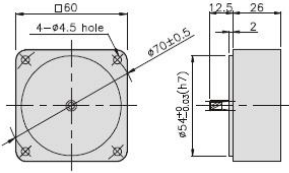
DECIMAL GEARHEAD K6G10BX \square
