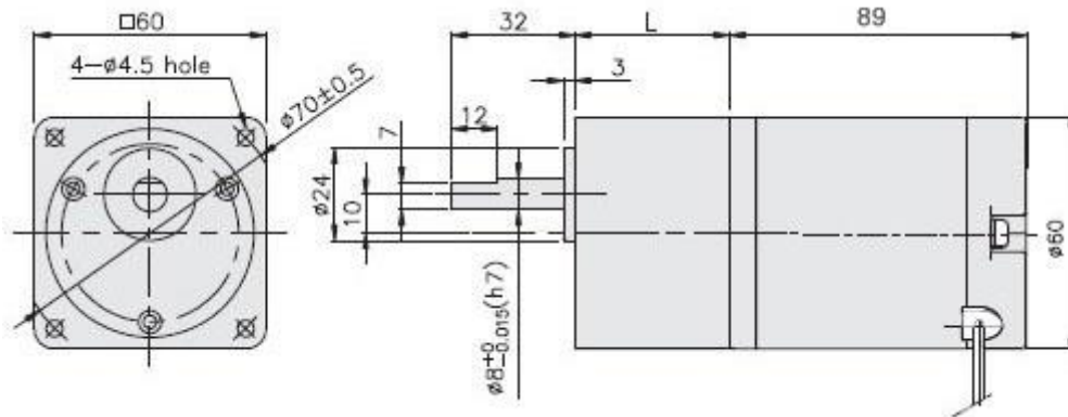
DG60-F \square 020B + K6G \square C
