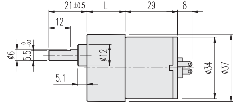
GEARHEAD LENGTH
